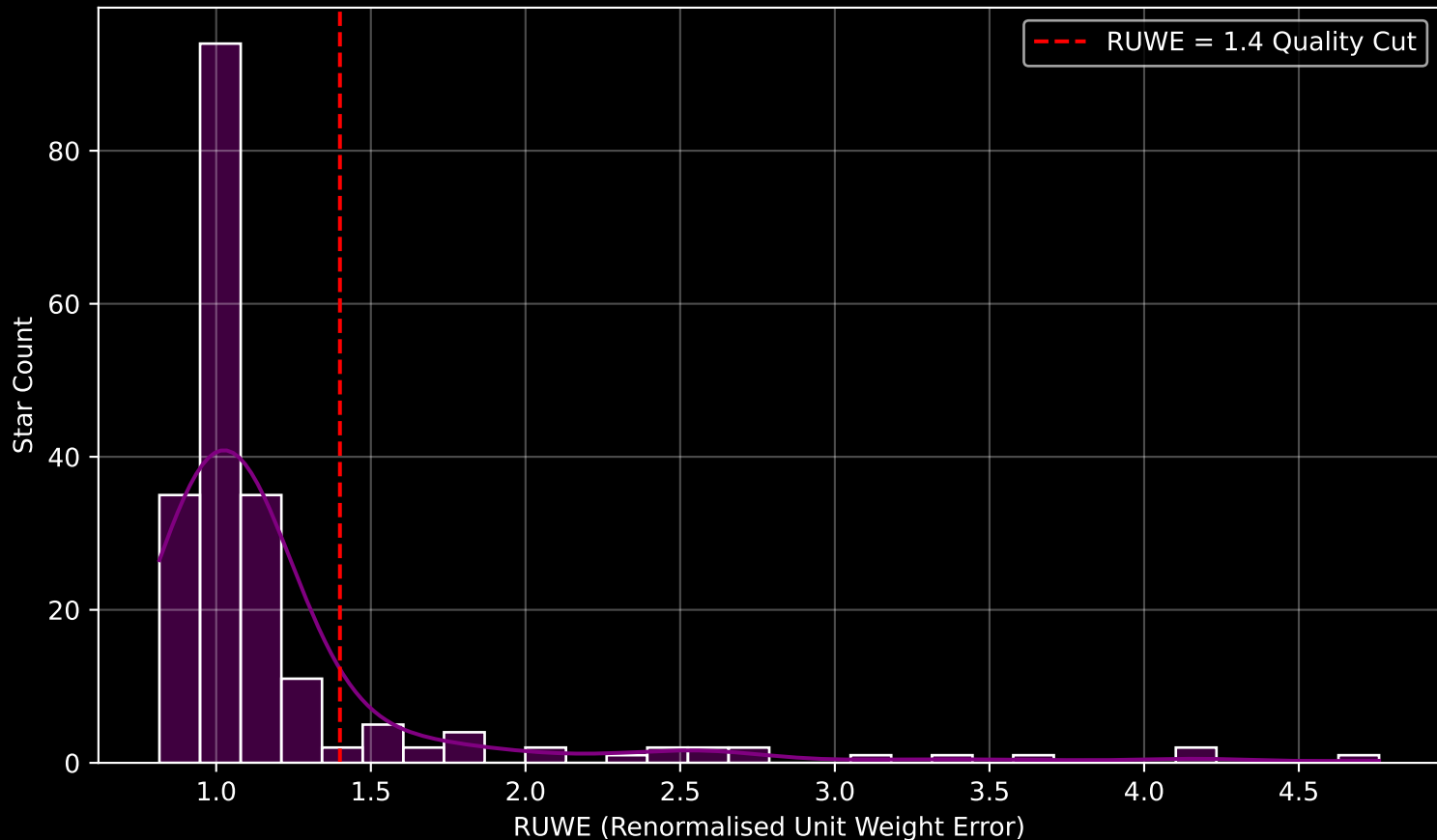
GAPOGEE DR17 Field [199+28] RUWE Distribution (n= 203)
