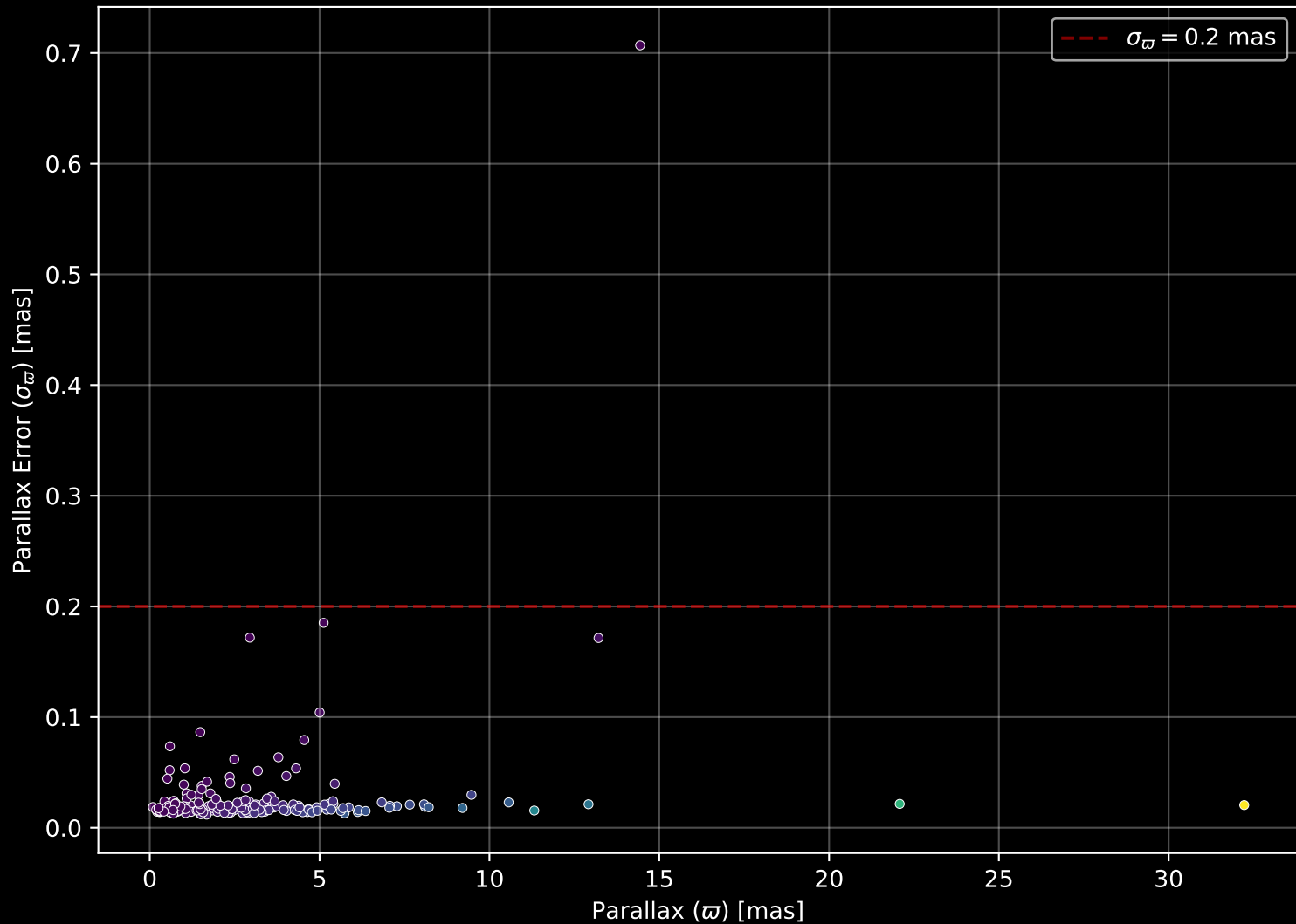
APOGEE DR17 Field: [199+28] Parallax Quality (n= 210)
