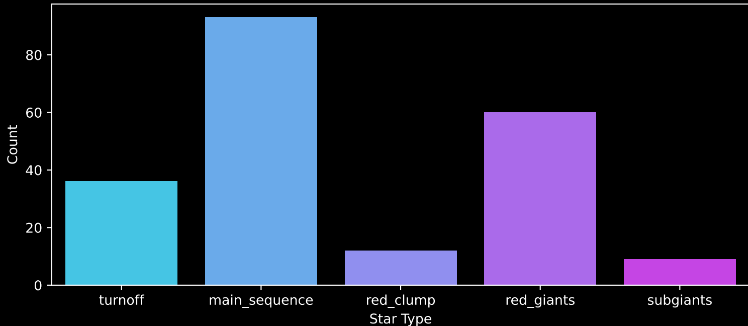
APOGEE DR17 Field: [199+28] Count plot of Star Type
