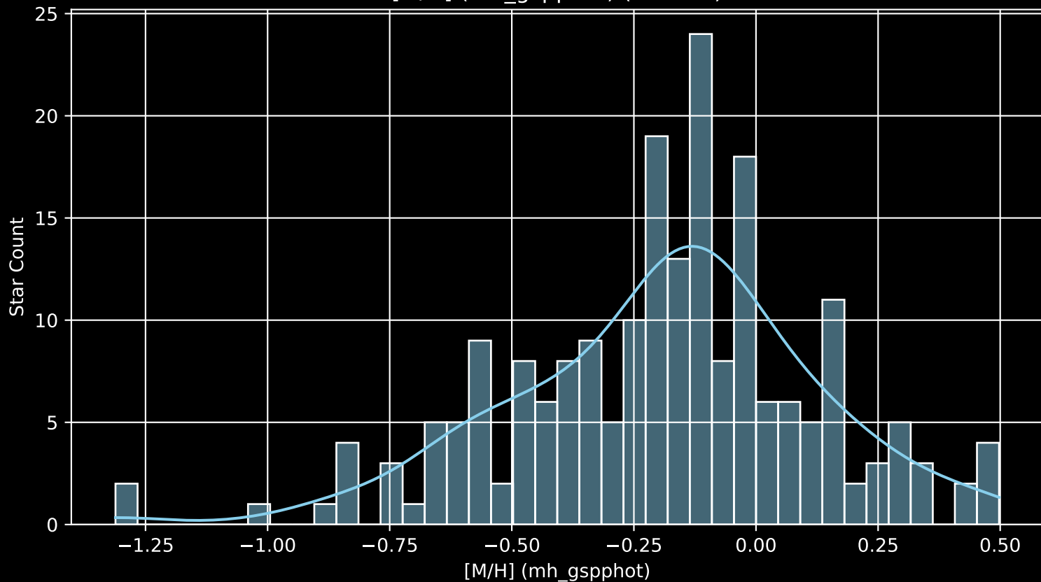
APOGEE DR17 Field: [199+28 [M/H] (mh_gspphot) (n= 208)
