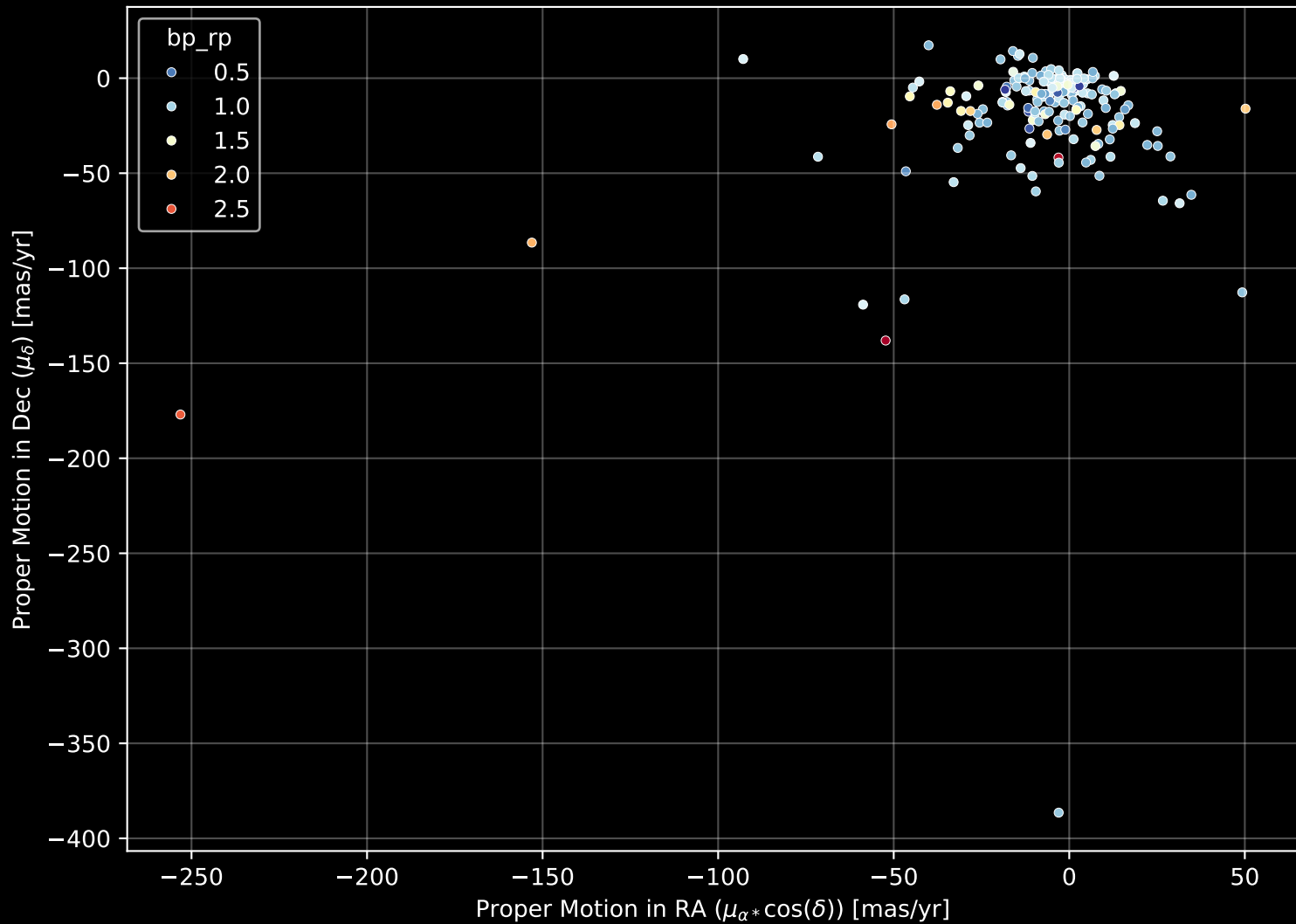
APOGEE DR17 Field: [199+28] Proper Motion Diagram (n= 210)
